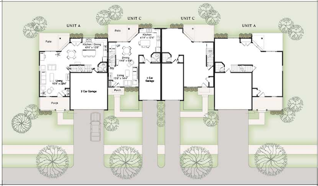
Floor Plan
